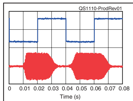
Figure 1 — CW keying waveform for the IC-7410 showing the first two dits in full break-in (QSK) mode using external keying. Equivalent keying speed is 60 WPM. The upper trace is the actual key closure; the lower trace is the RF envelope. (Note that the first key closure starts at the left edge of the figure.) Horizontal divisions are 10 ms. The transceiver was being operated at 100 W output on the 14 MHz band.
