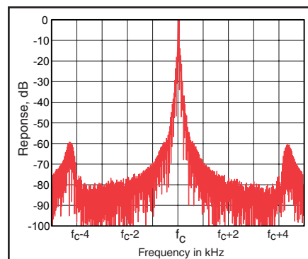
Figure 2 — Spectral display of the IC-7410 transmitter during keying sideband testing. Equivalent keying speed is 60 WPM using external keying. Spectrum analyzer resolution bandwidth is 10 Hz, and the sweep time is 30 seconds. The transmitter was being operated at 100 W PEP output on the 14 MHz band. This plot shows the transmitter output \pm 5 kHz from the carrier. The reference level is 0 dBc, and the vertical scale is in dB. Note that the keying sideband level rises slightly at the edges, to the -60 dB range.
